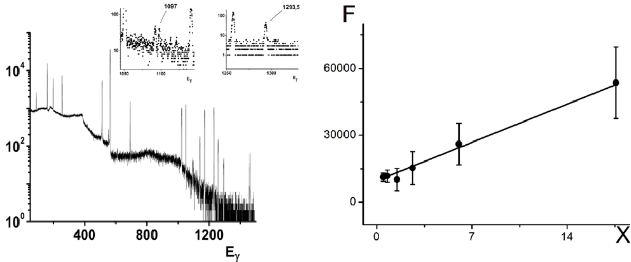
Figure 1. Gamma-ray spectra from the antimony activities. The analytical gamma lines used for determination of the isomer ratios are indicated separately (left). Fitting line for experimental points (X, F) of antimony ^{116m,g}\text{Sb} nuclei decay (reaction ^{121}\text{Sb}(\gamma,5n)^{116m,g}\text{Sb} ) (right).
