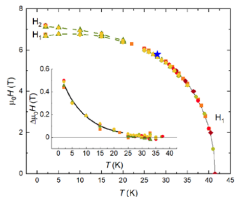
U\text{IrSi}_3 phase diagram complemented with acoustic data [2] (grey color existing diagram [1]).
