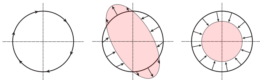
Figure 3.3: Schematic visualization of the optical scalars effects on a null geodesic congruence in terms of the twist (left), shear (middle), and expansion (right).
