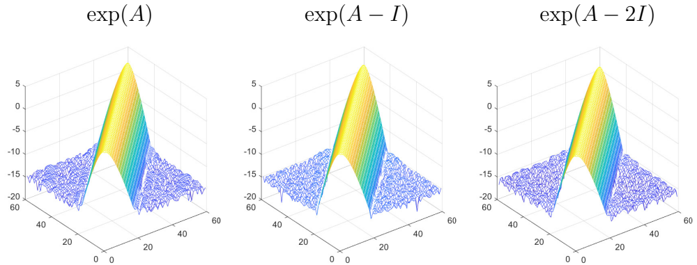
Figure 1.2: Magnitude of the matrix exponential elements (logarithmic scale). The matrix A is the same as in Figure 1.1.
